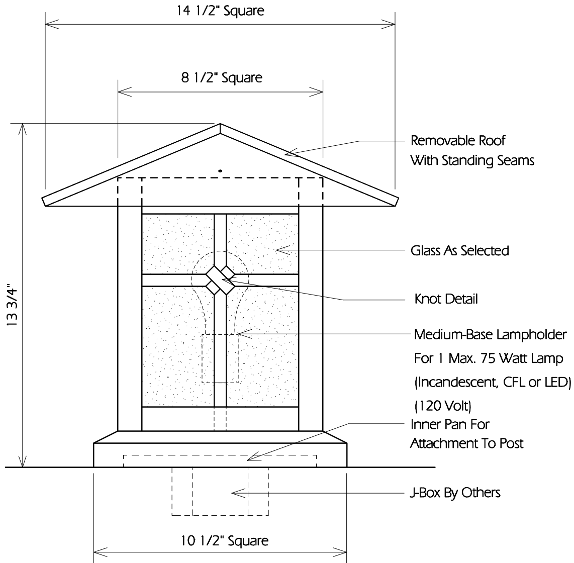
TYPICAL SIDE
