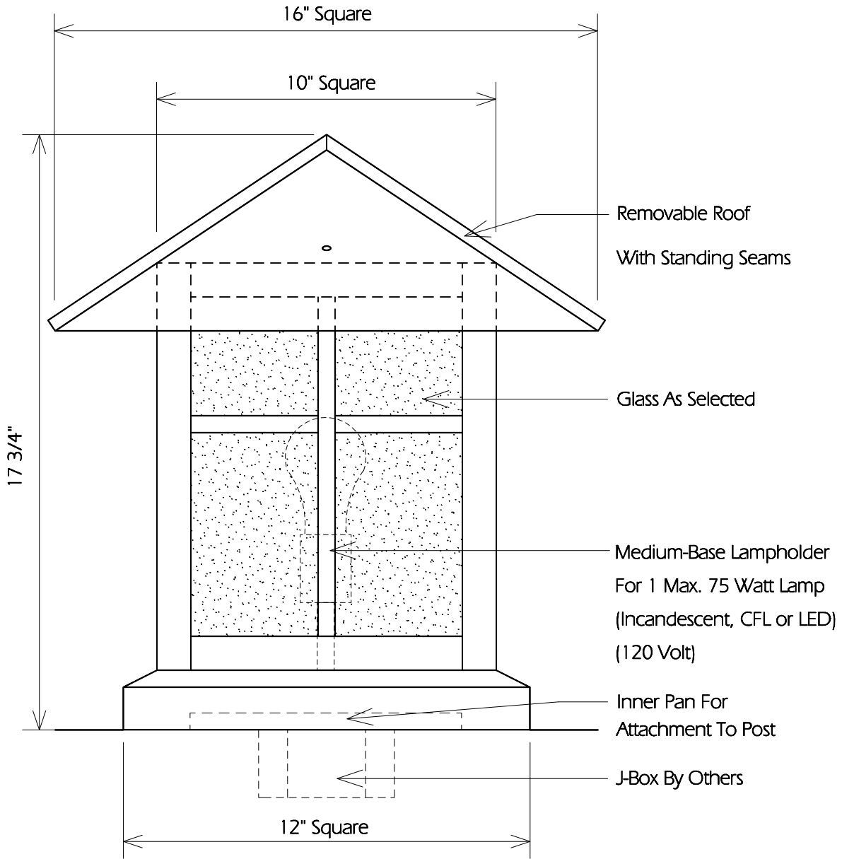
TYPICAL SIDE
