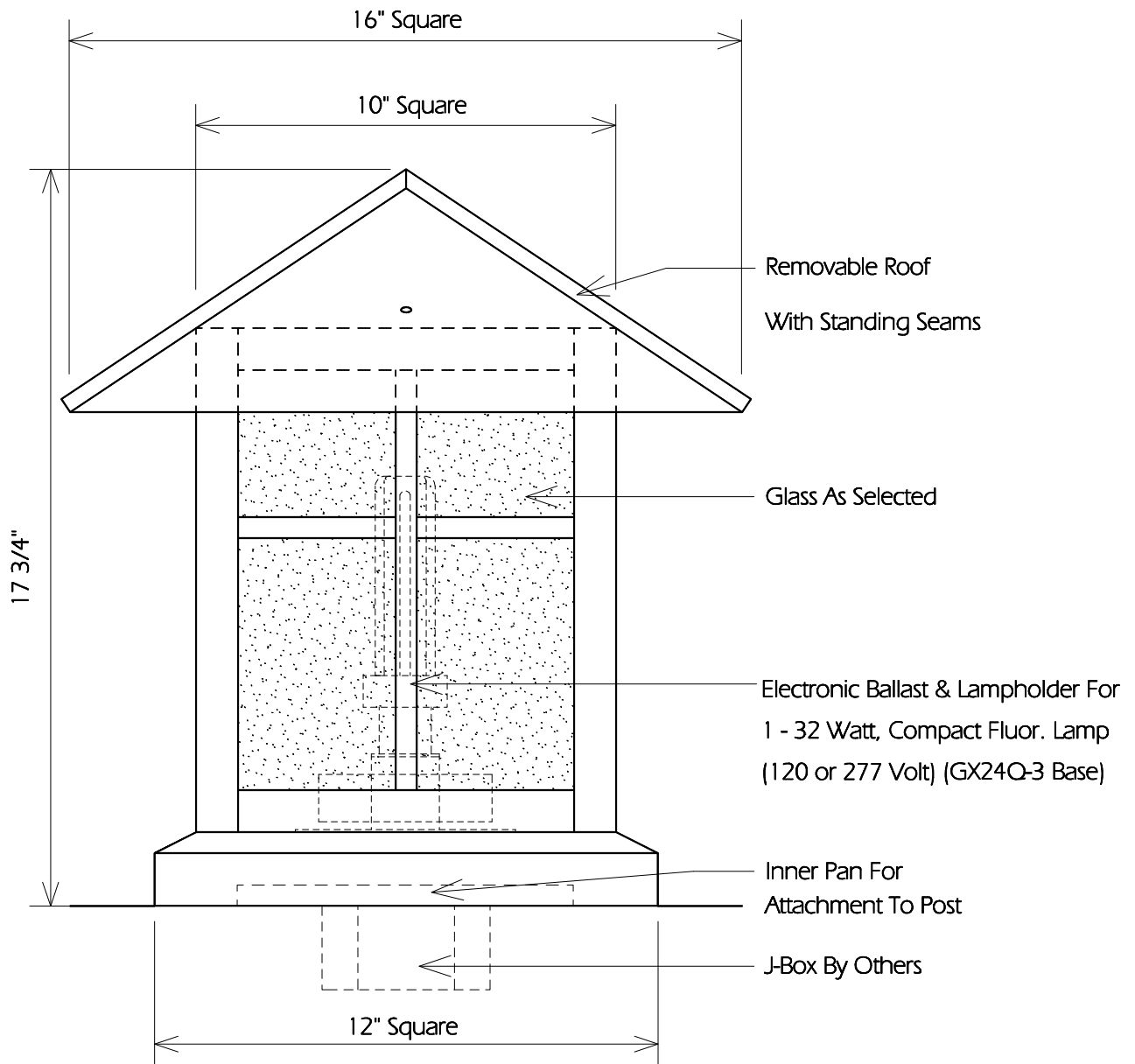
TYPICAL SIDE
