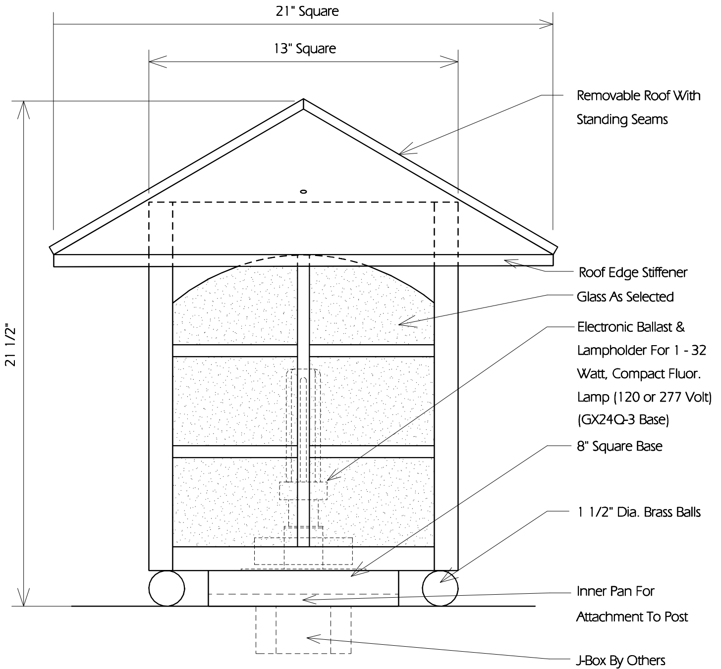
TYPICAL SIDE
