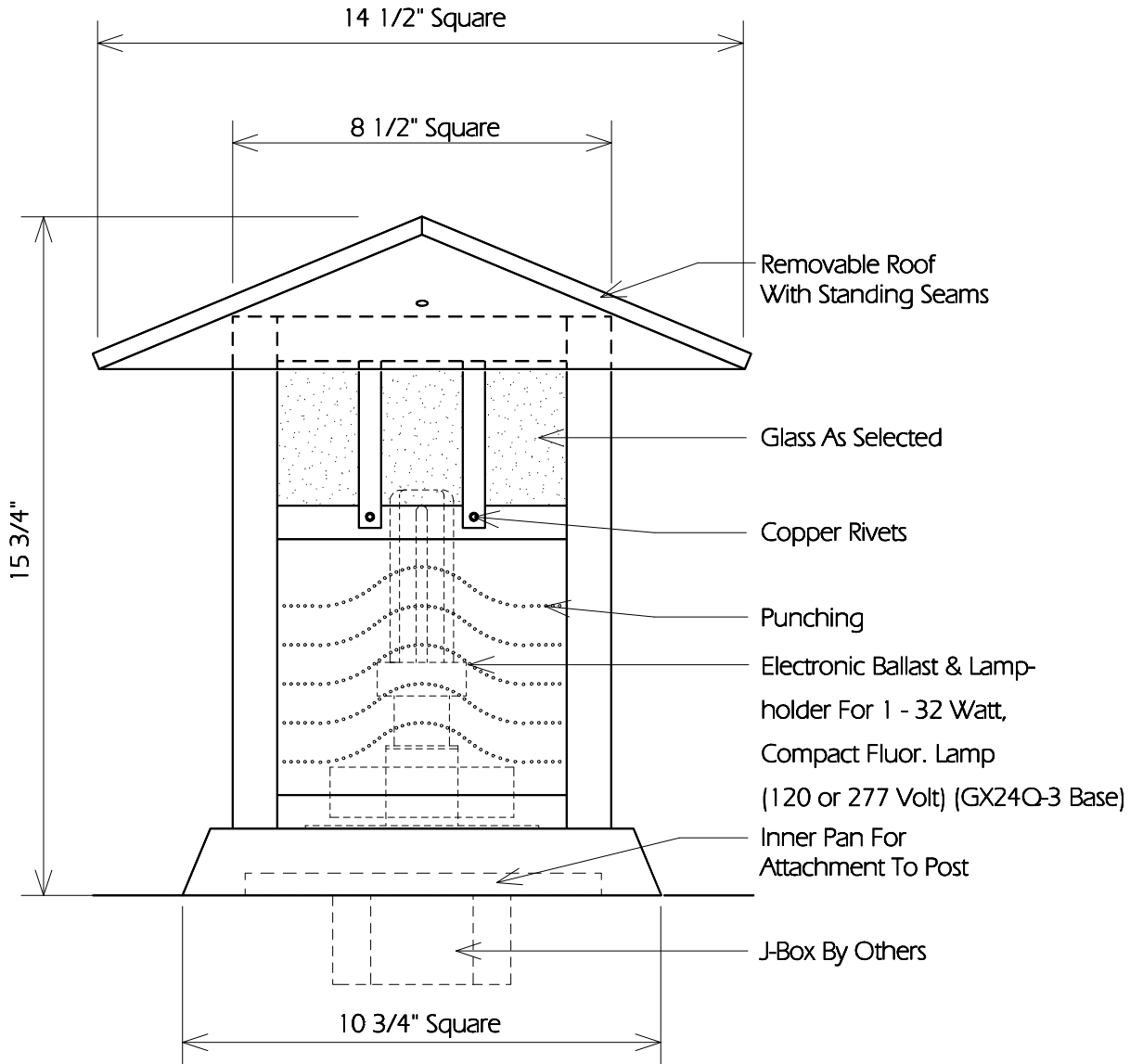
TYPICAL SIDE
