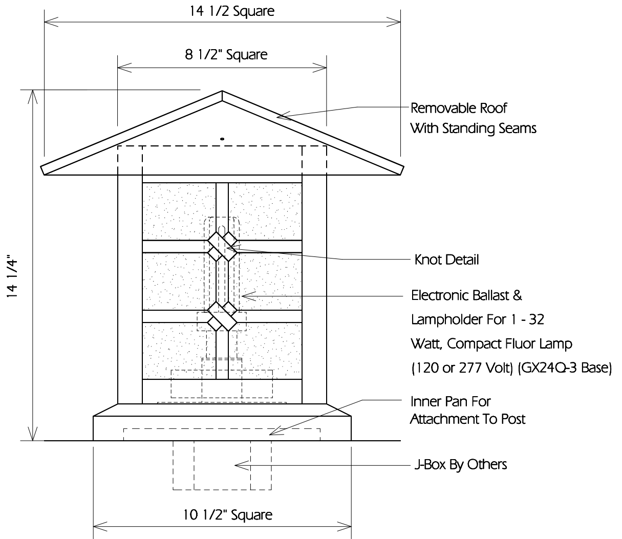
TYPICAL SIDE
