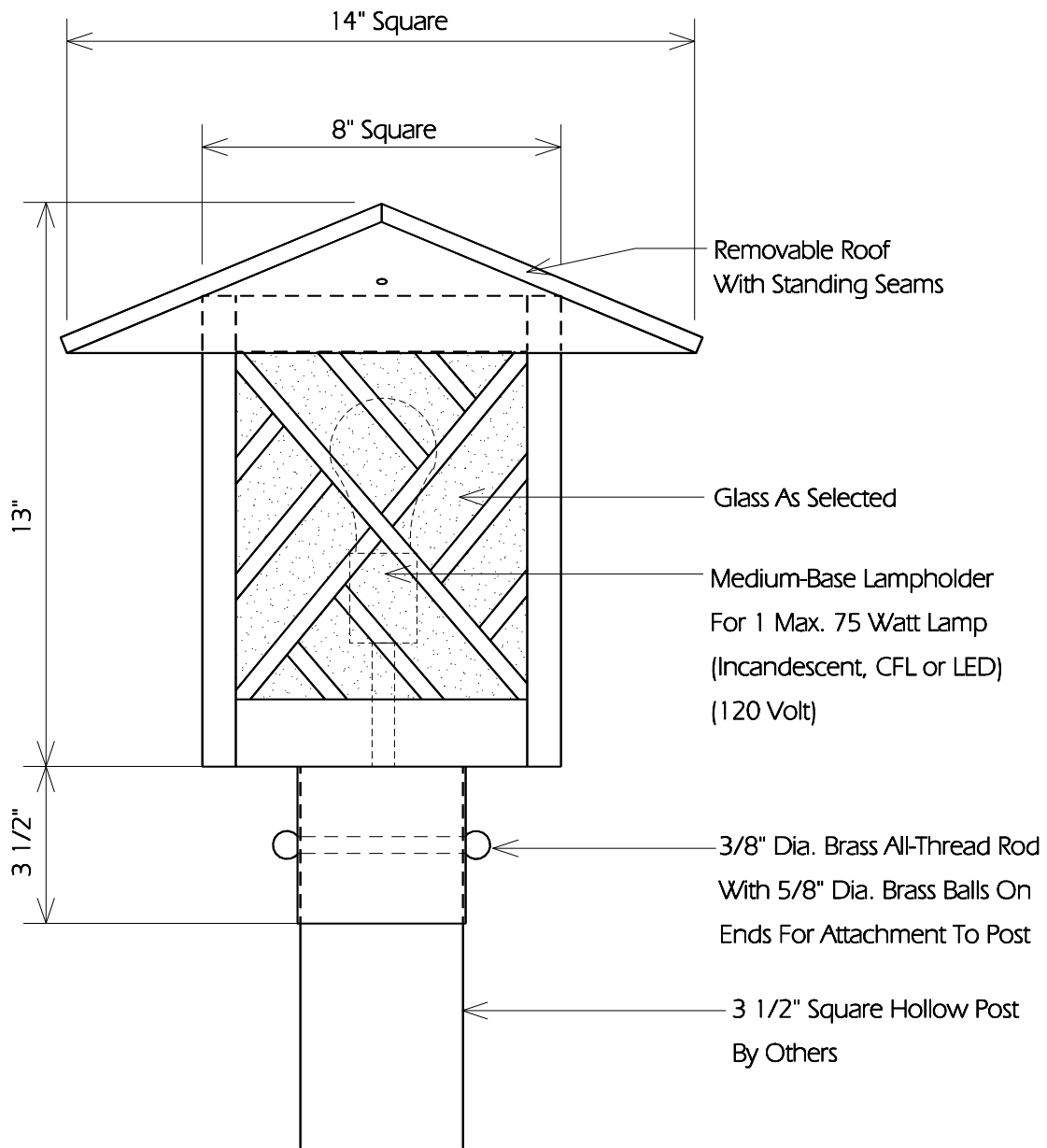
TYPICAL SIDE
