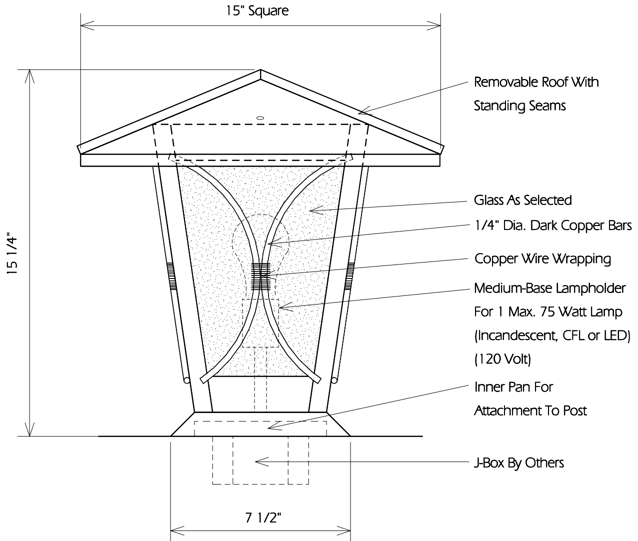
TYPICAL SIDE
