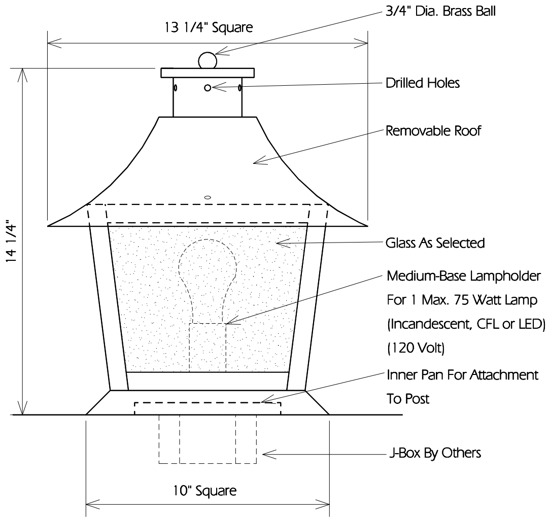
TYPICAL SIDE
