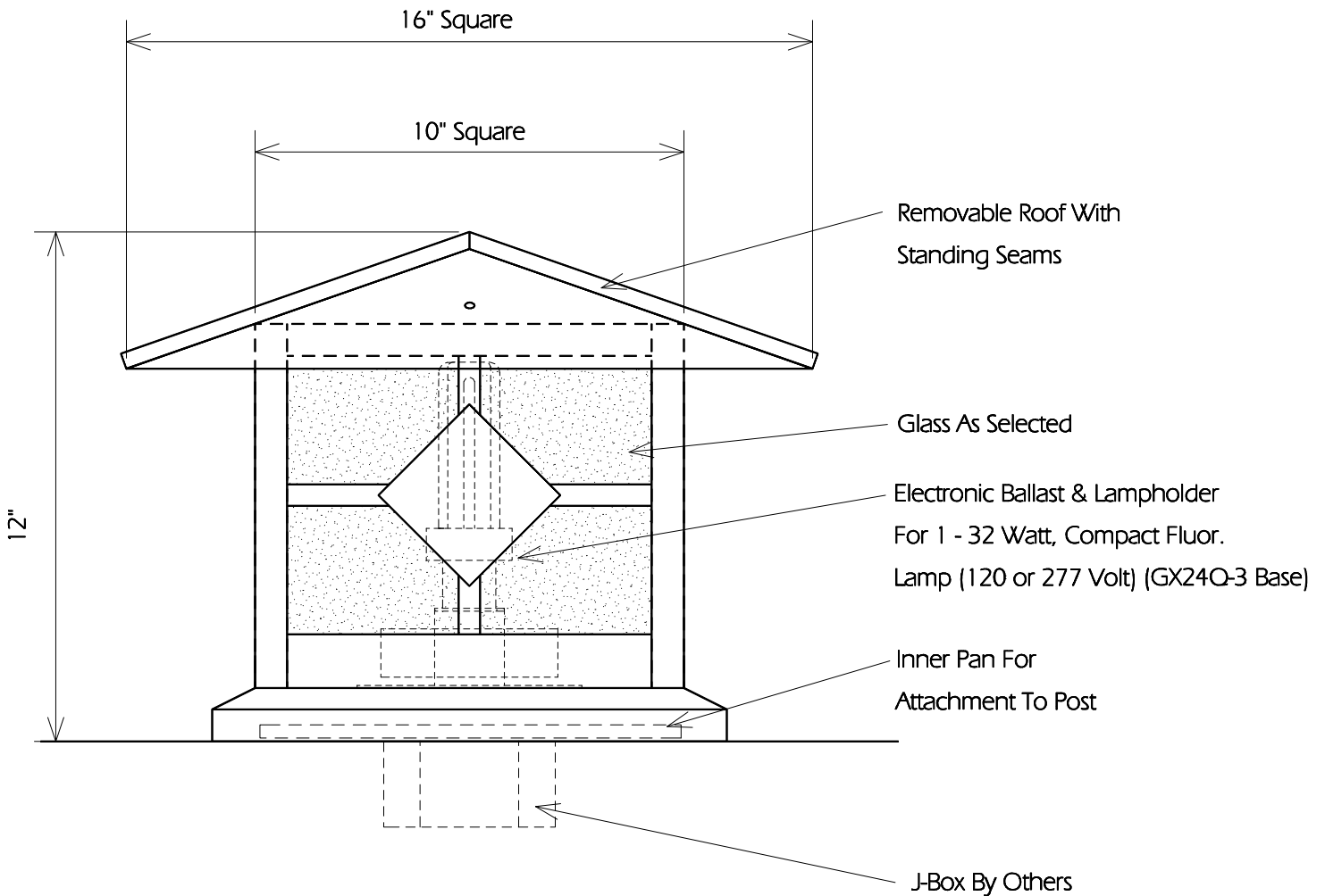
TYPICAL SIDE
