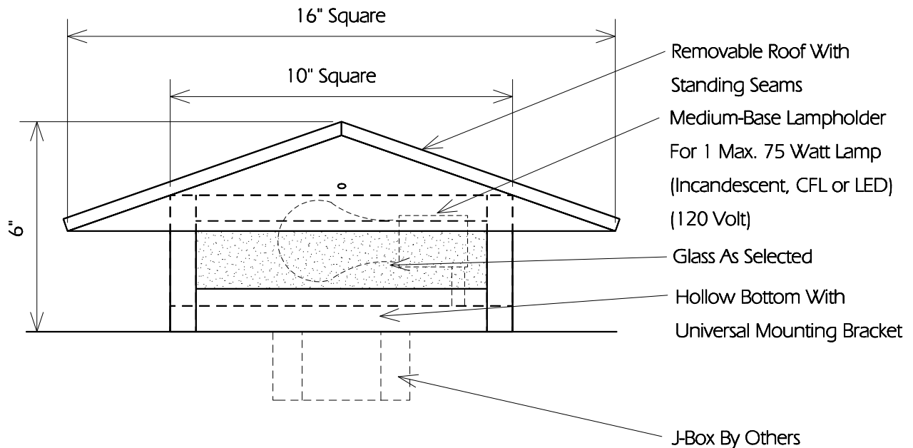
TYPICAL SIDE
