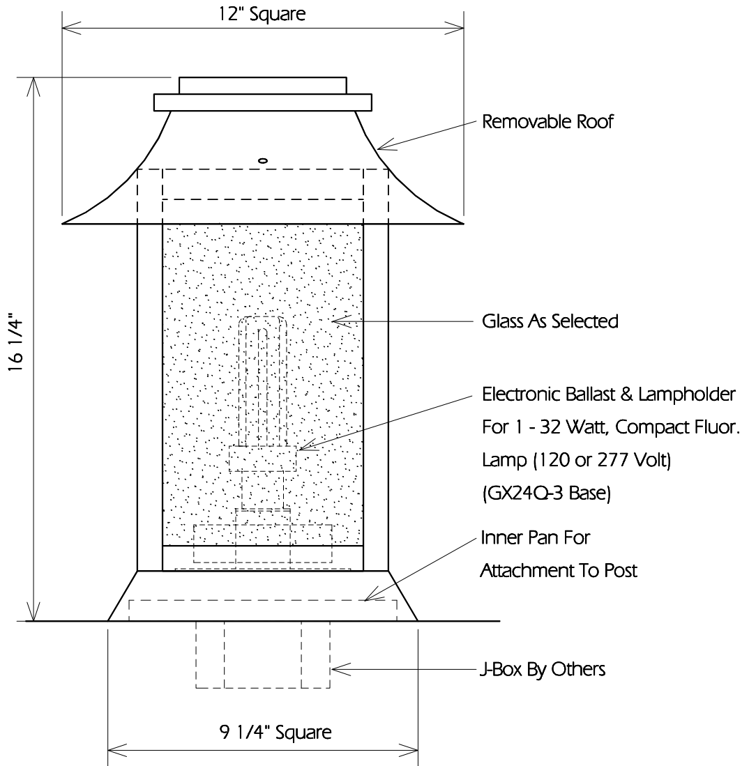
TYPICAL SIDE
