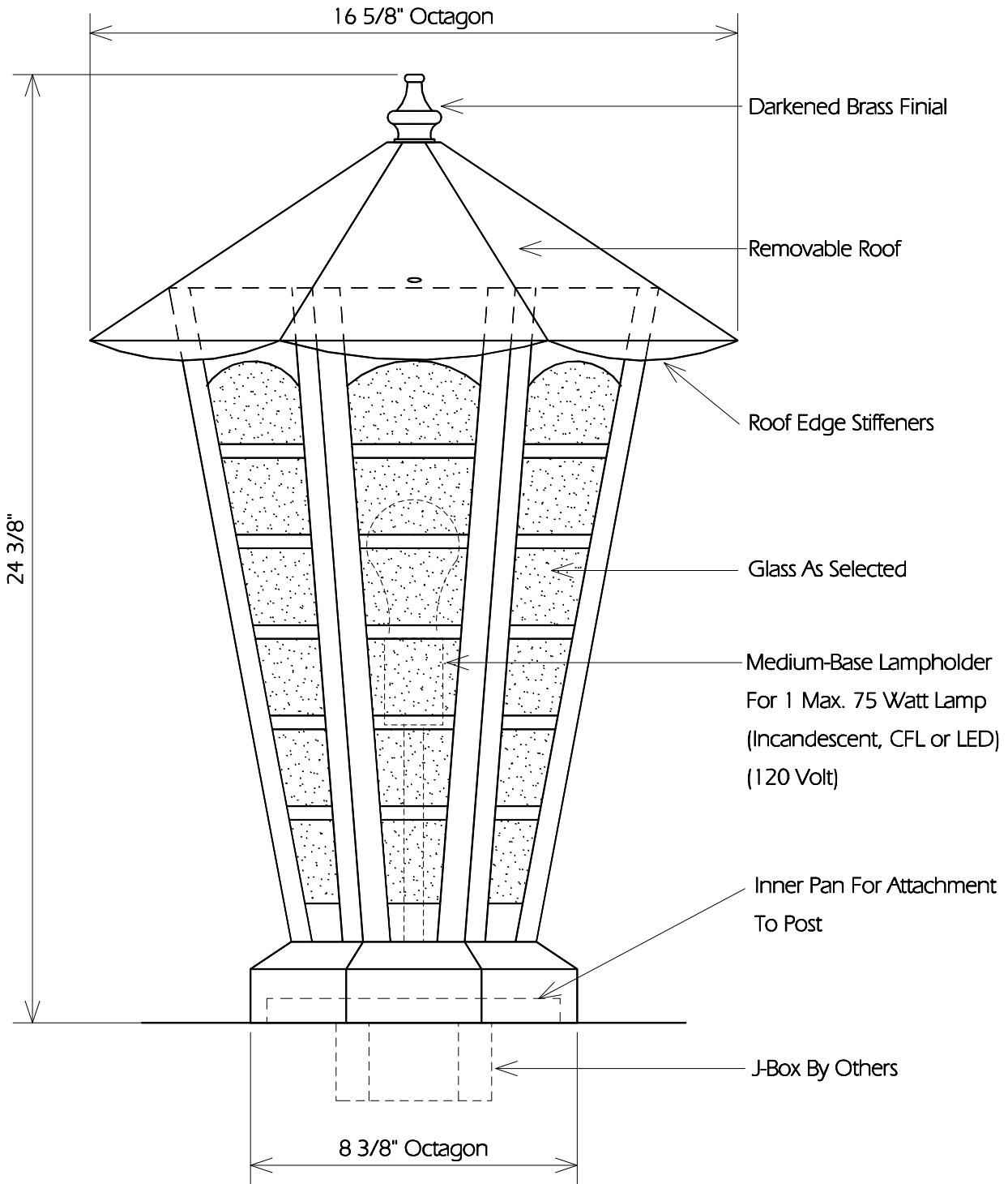
TYPICAL SIDE
