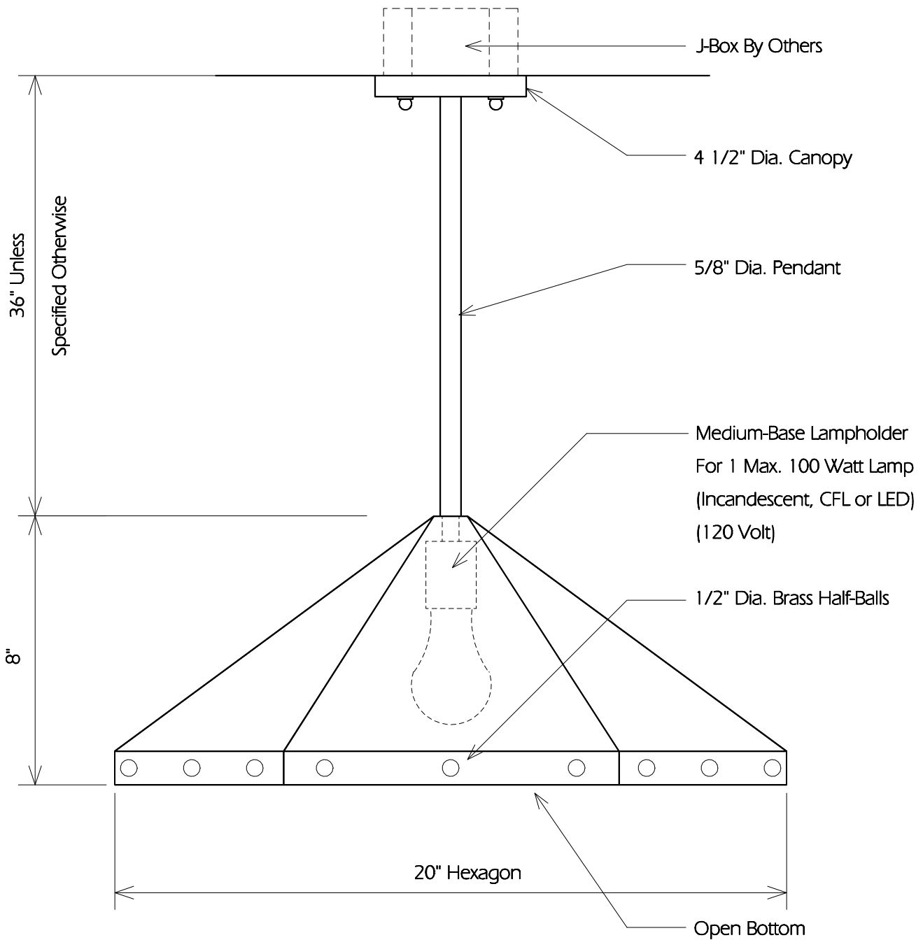
TYPICAL SIDE
