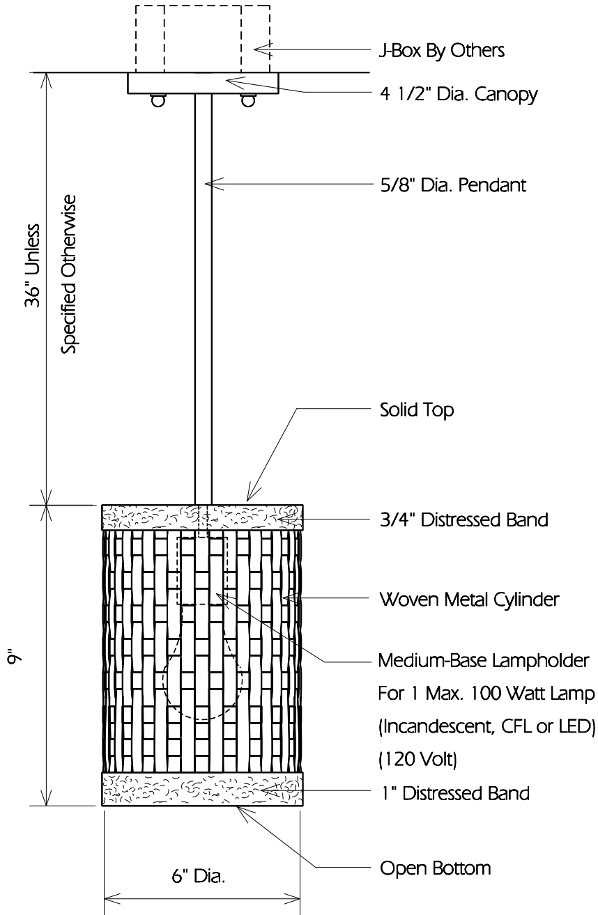
TYPICAL SIDE
