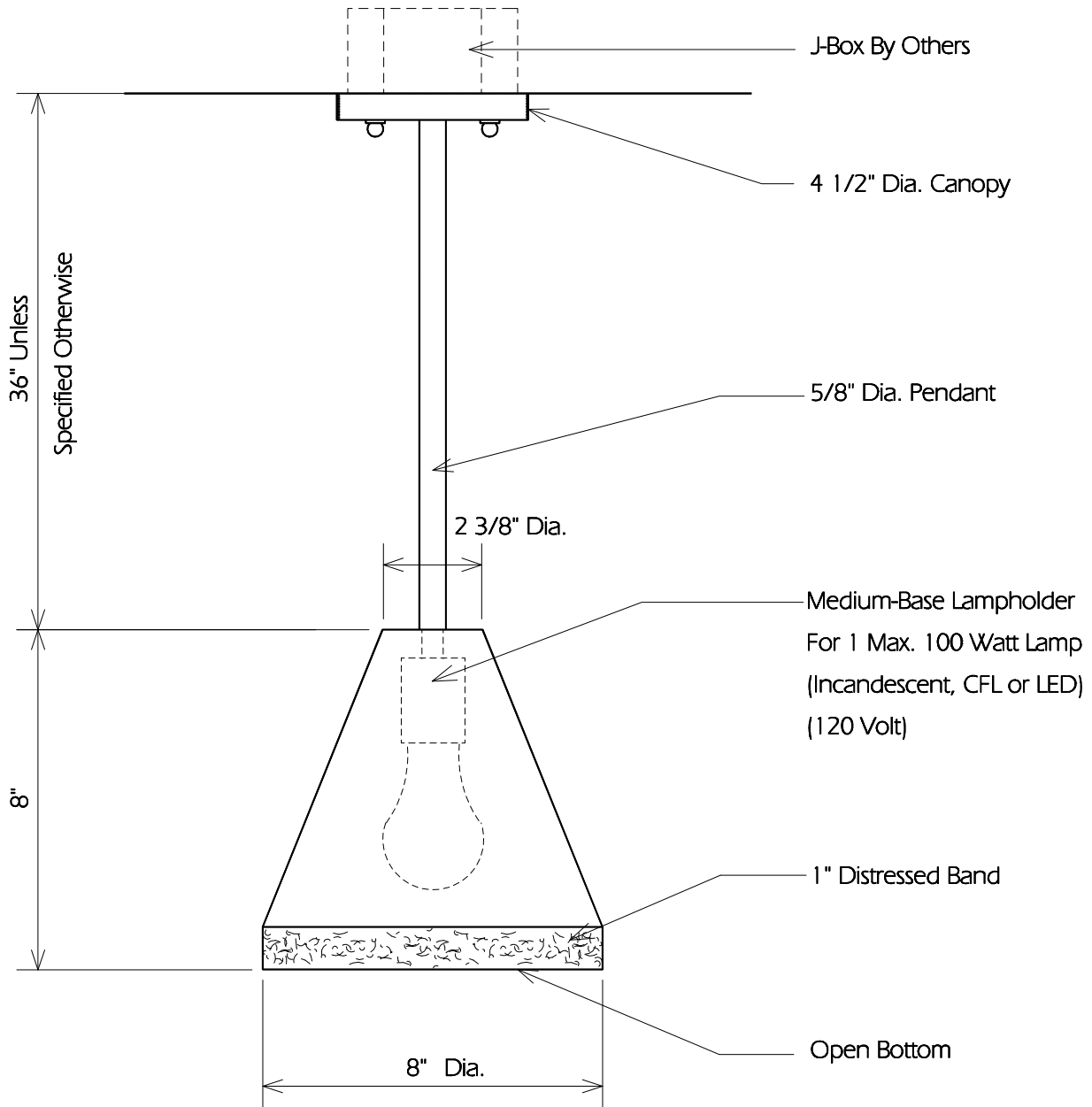
TYPICAL SIDE
