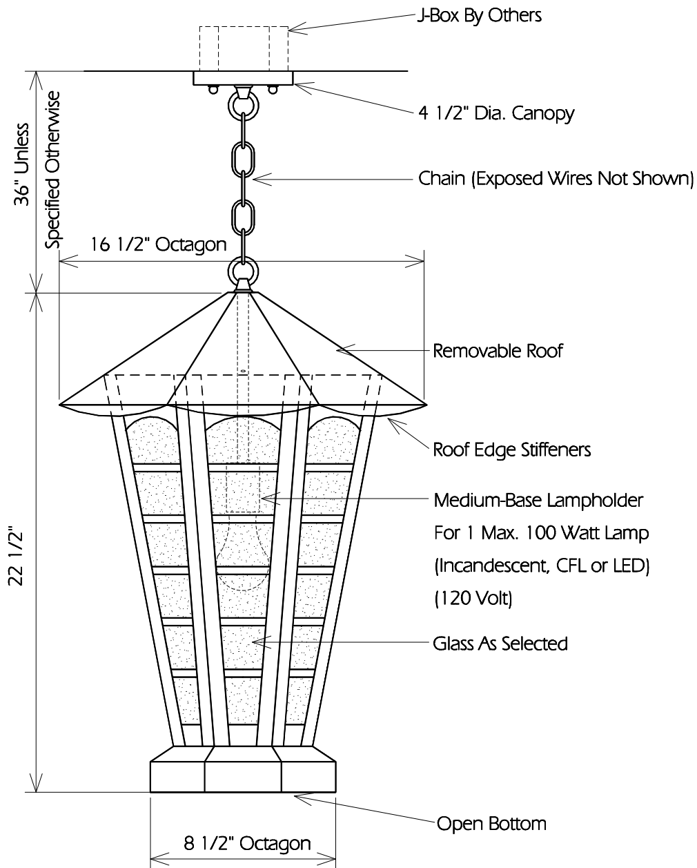
TYPICAL SIDE
