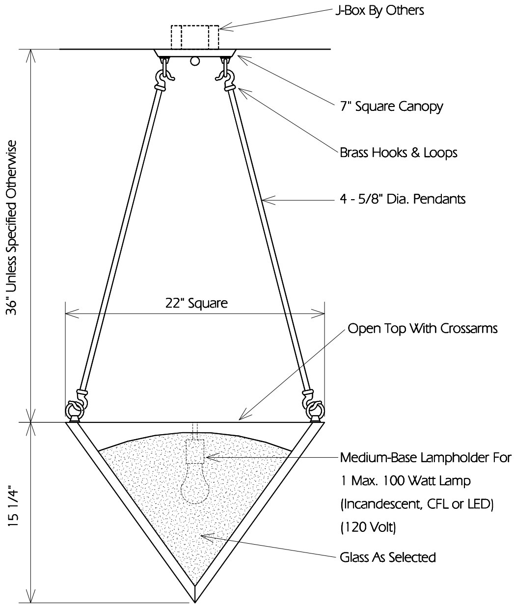
TYPICAL SIDE
