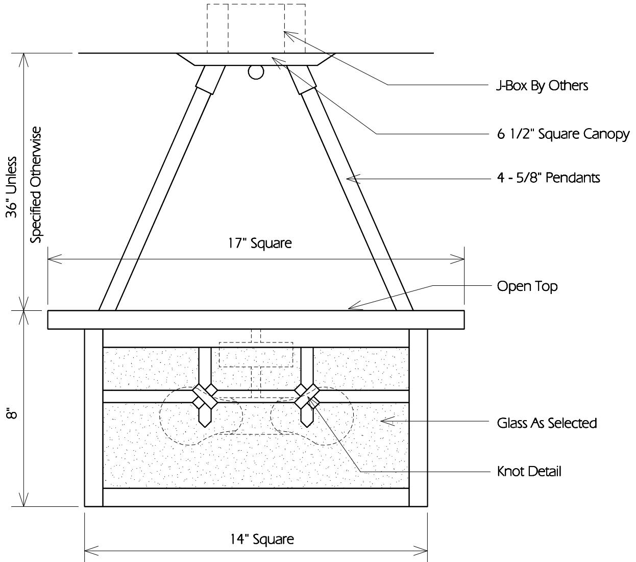
TYPICAL SIDE
