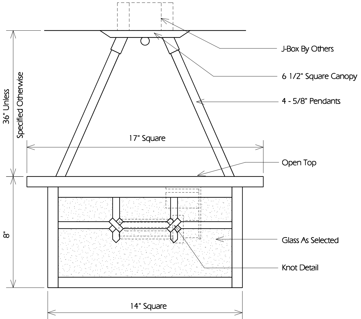
TYPICAL SIDE
