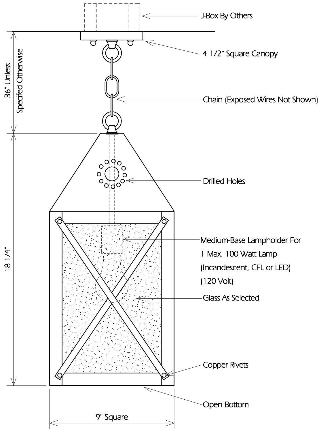
TYPICAL SIDE
