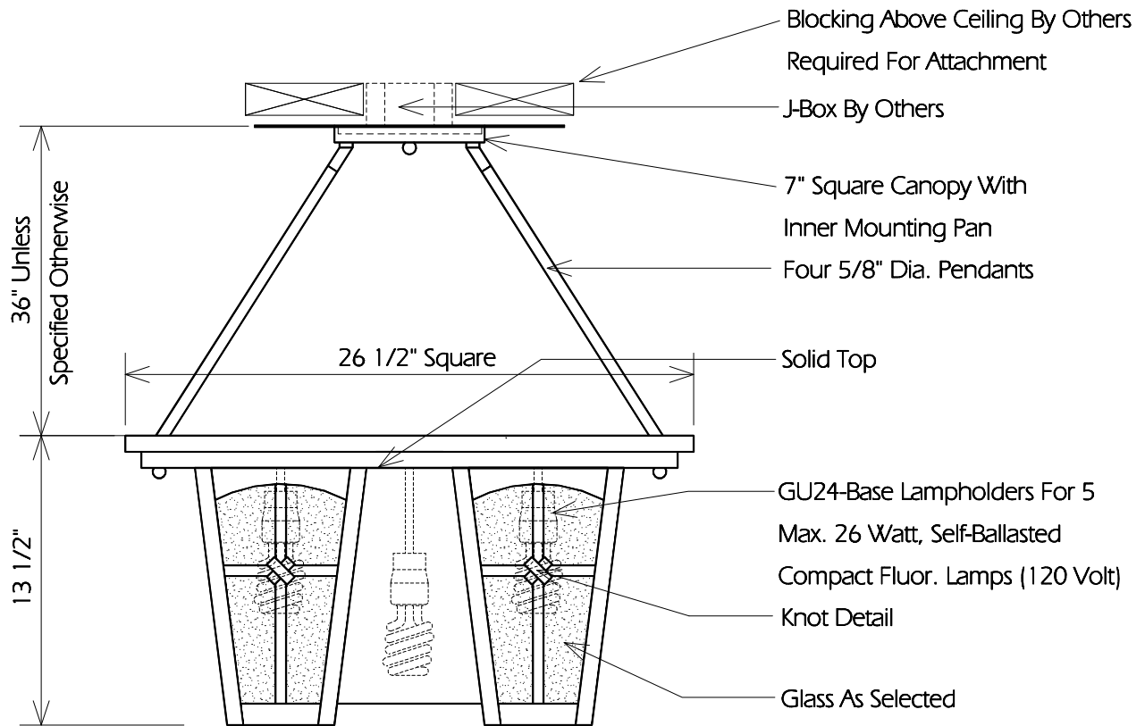
TYPICAL SIDE
