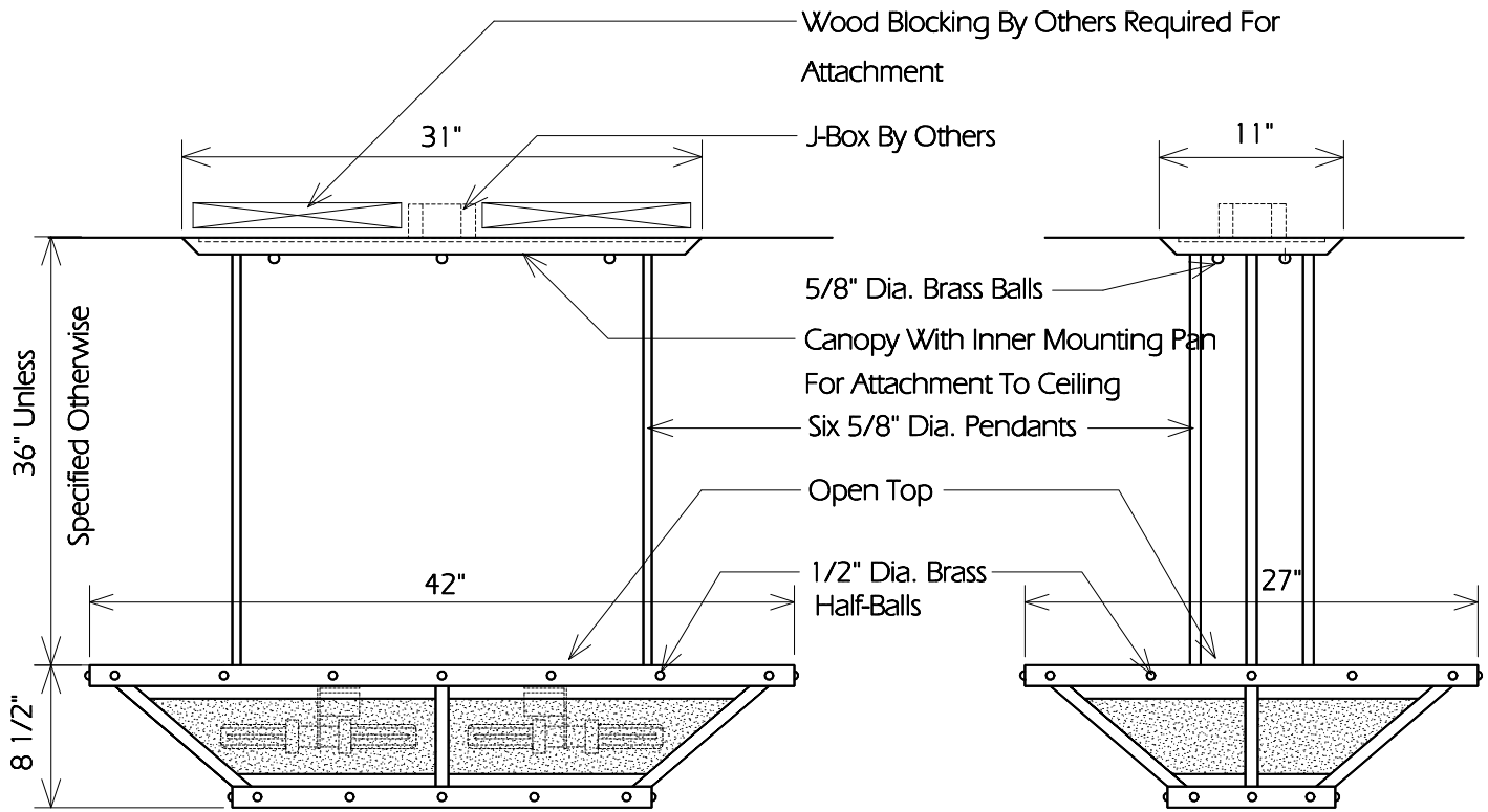
SIDE
