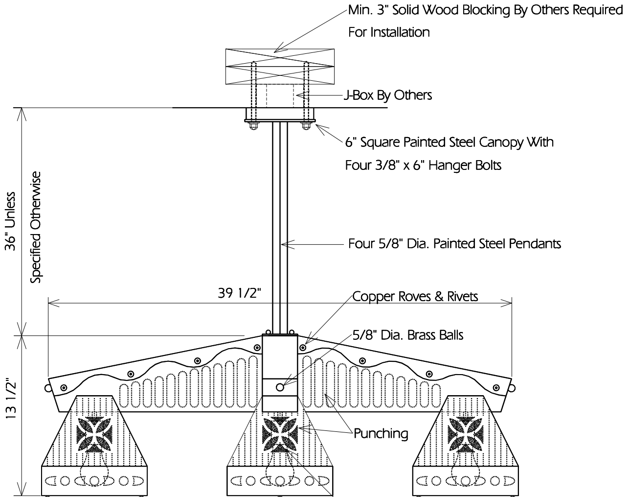
TYPICAL SIDE
