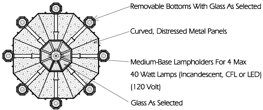
BOTTOM (Shown Half Size)
