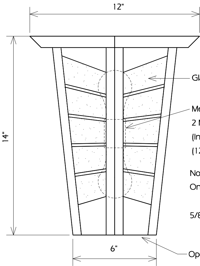
FRONT
