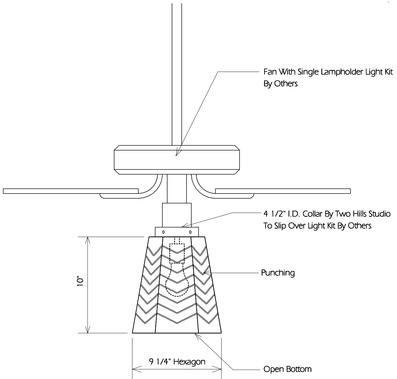
TYPICAL SIDE
