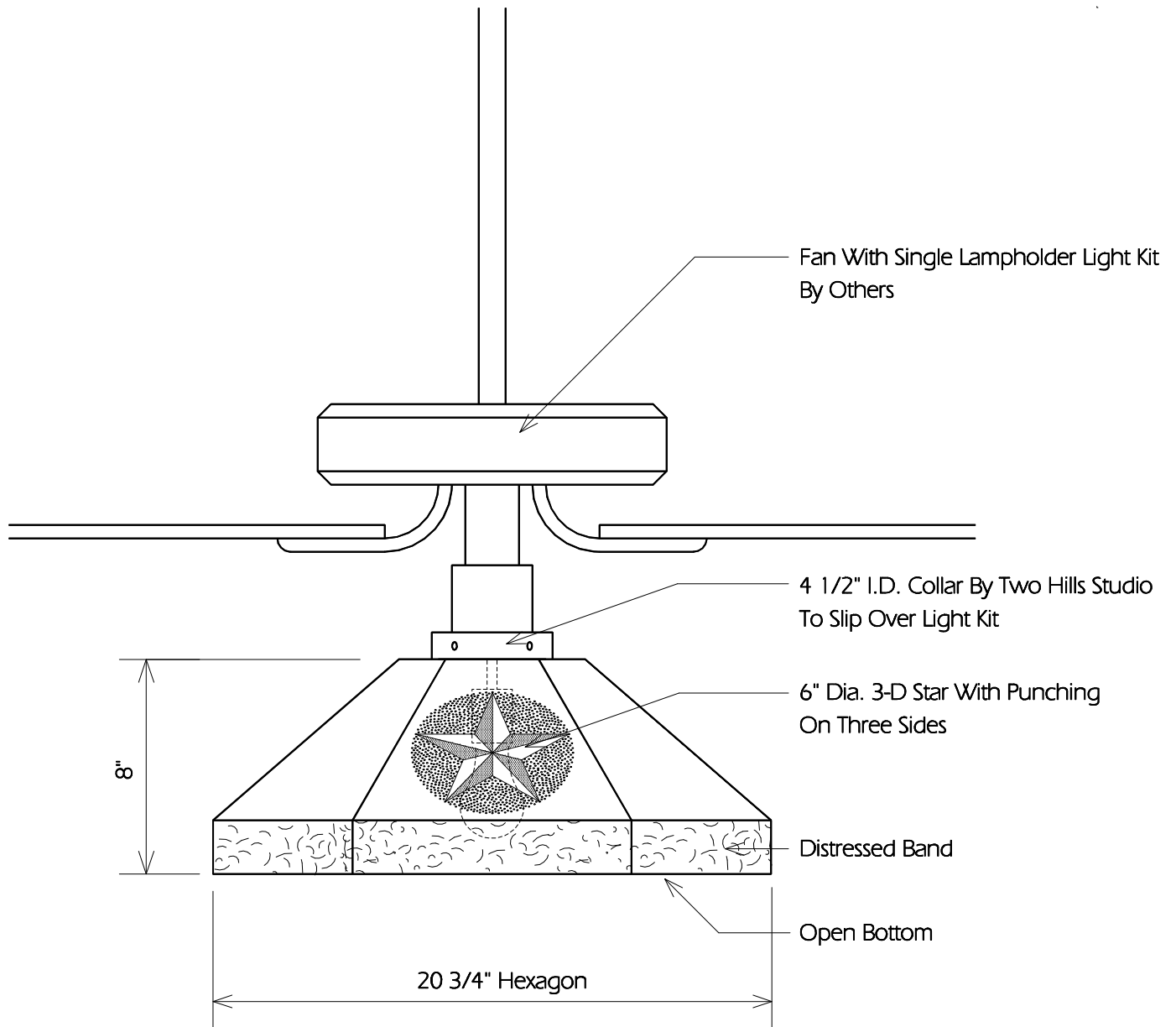
TYPICAL SIDE
