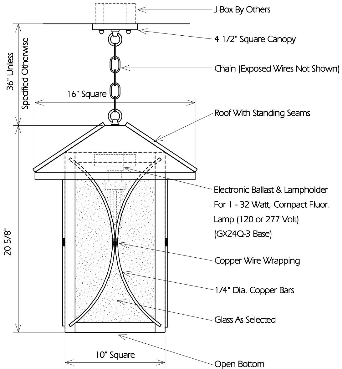
TYPICAL SIDE
